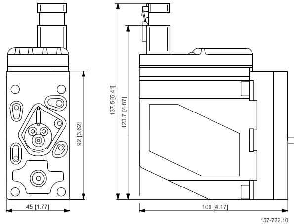
PVE with Deutsch® connector incl. female connector
