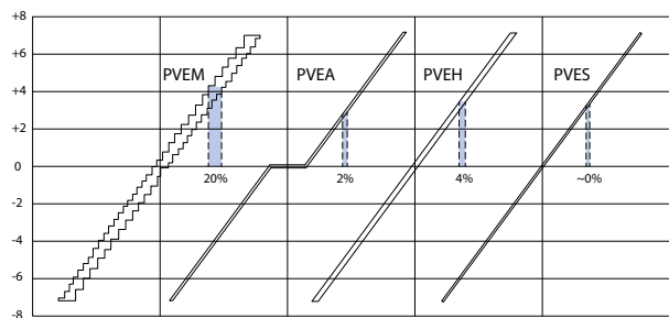
Hysteresis for PVE variants*
