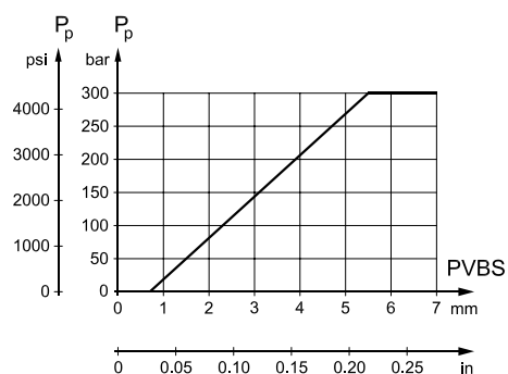
Pump pressure vs. spool travel curve
